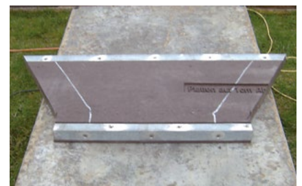
Trimmed and subsequently reinforced shim plate.
